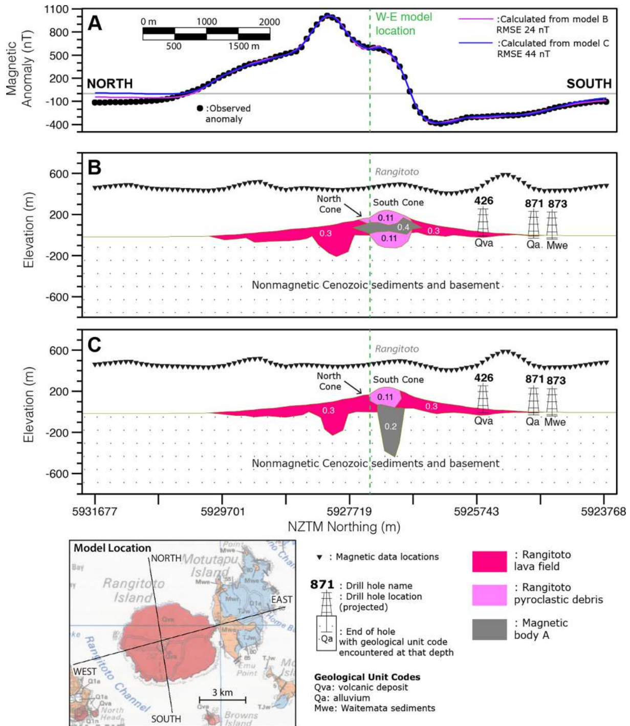
Fig. 8. (A) Observed and calculated magnetic anomaly data of north–south Rangitoto Island transect. Grey line marks 0 nT. (B) and (C) are two endmembers of the 2.5D models of subsurface susceptibility distribution below the transect. Legend and locator map to the models are below (C). True offline well and data point elevations have been projected onto the 2D topographic surface shown.
