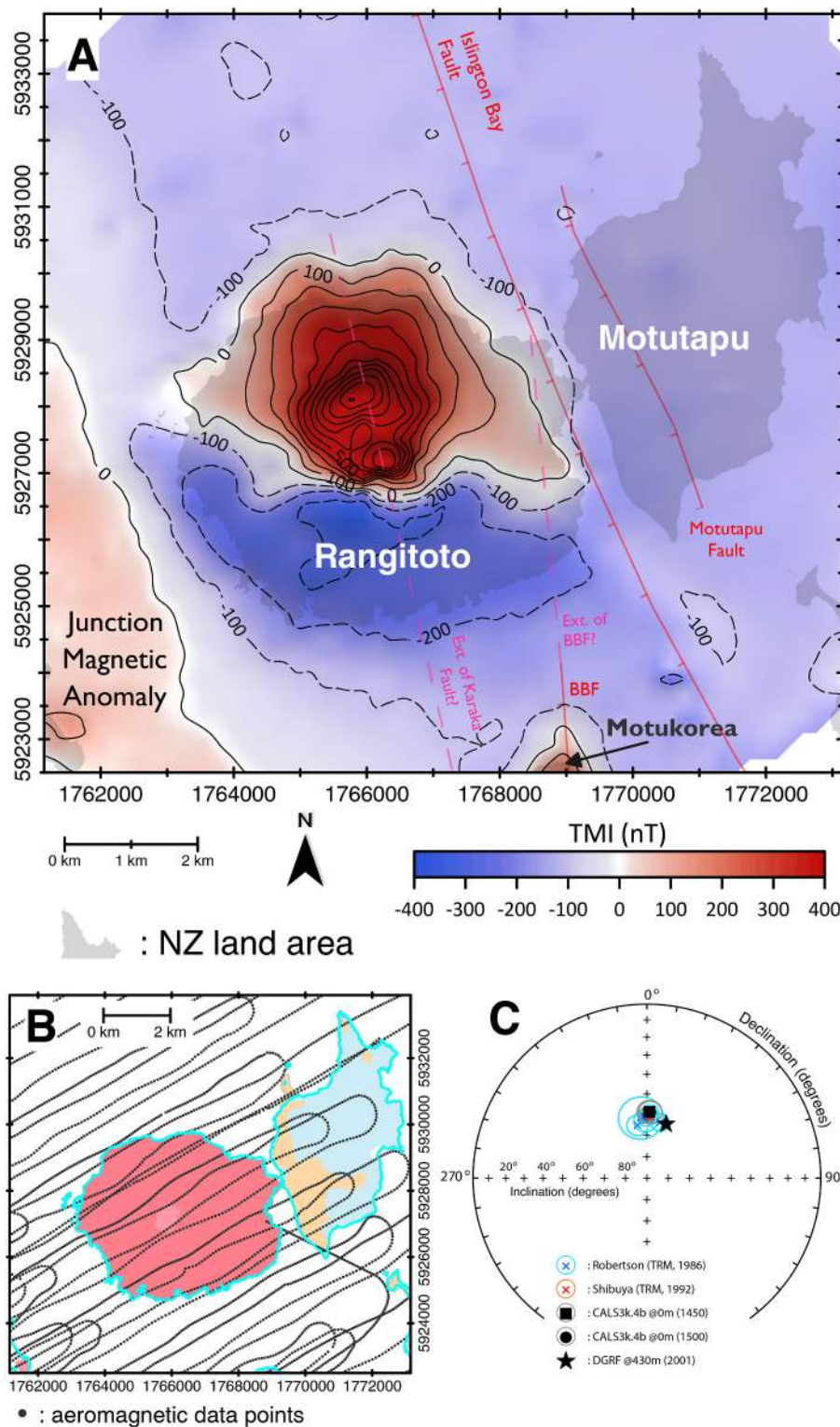
Fig. 4. (A) Magnetic anomaly map of the Rangitoto and Motutapu Islands. Contour lines every 100 nT, and BBF stands for Bucklands Beach Fault. (B) The location of the aeromagnetic data points, plotted on the geological map of Rangitoto and Motutapu. For colour legend, please refer to Fig. 1C. (C) Equal-area plot of Rangitoto basalt paleo-inclination and declination (acquired from thermoremanent magnetisation, TRM) with the modelled Rangitoto geomagnetic inclination and declination in 1450, 1500, and 2001 AD. The Rangitoto geomagnetic parameters for the year 1450 and 1500 AD are calculated on the earth surface using the CALS3k.4b model (Korte and Constable, 2011). DGRF epoch 2000 coefficients are used for calculating the 2001 AD geomagnetic parameters at 430 m above Rangitoto, the aeromagnetic flight level (Alken et al., 2021; Eccles et al., 2005). Paleomagnetic data is marked with cross, modelled values are marked with filled shapes, and 95% confidence ellipses are indicated. All inclination values are negative.
