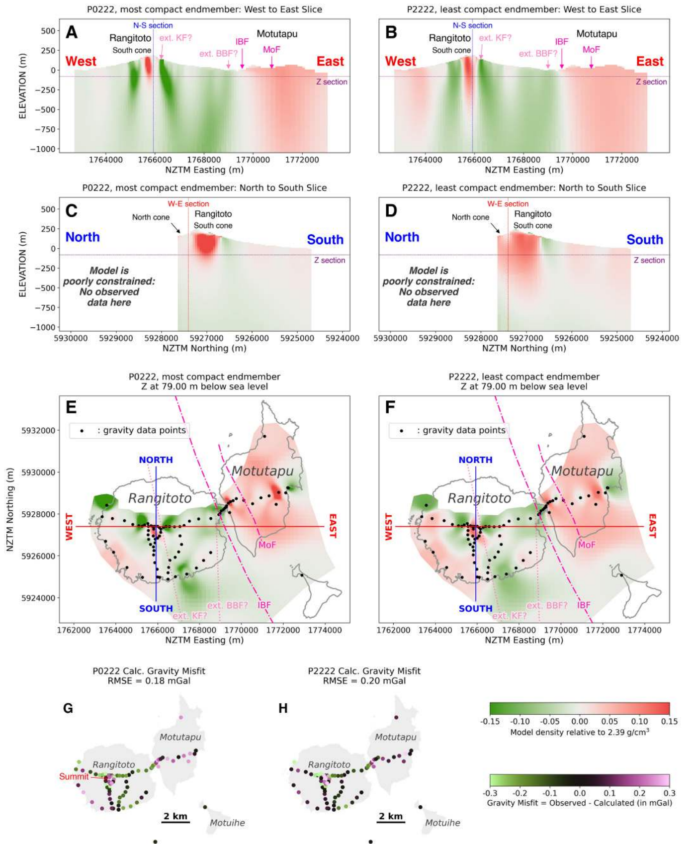
Fig. 9. 3D gravity model of Rangitoto subsurface. Figures (A, C, E) represent the west-east, north-south, and vertical slices of compact endmember ( p\text{-norm} = 0 ) of the gravity 3D models. Vertical slice is made at 79 m below sea level. Compare figures (A, C, E) with figures (B, D, F) from the smooth ( p\text{-norm} = 2 ) gravity model endmember. Figures (G) and (H) are the data misfit maps of the compact and smooth models, respectively. IBF: Islington Bay Fault, MoF: Motutapu Fault, ext. BBF?: extension of Bucklands Bay Fault (uncertain), ext. KF?: extension of Karaka Fault (uncertain).
