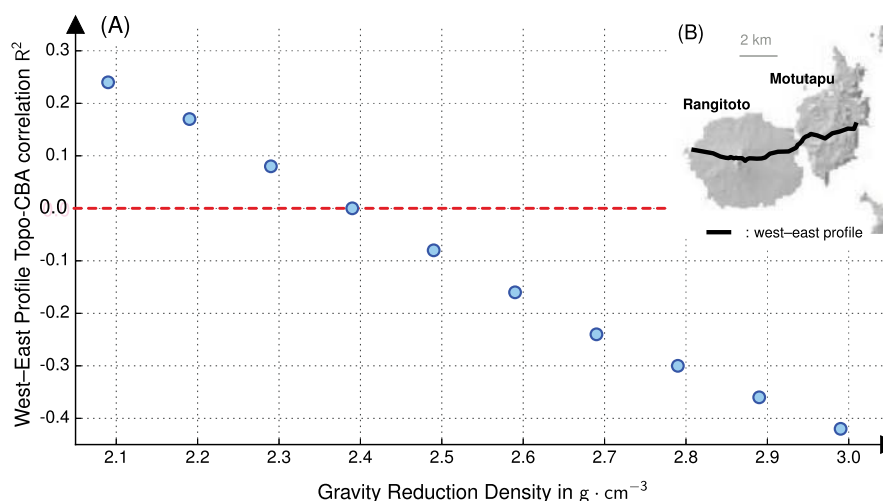
Fig. 2. (A) Pearson correlation R^2 between topographic variation and complete Bouguer anomaly along west-east profile on Rangitoto and Motutapu Islands (see inset B) as a function of reduction density. A density of 2.39 \text{ g/cm}^3 minimised the correlation of Bouguer anomaly with topography across the entire profile.
