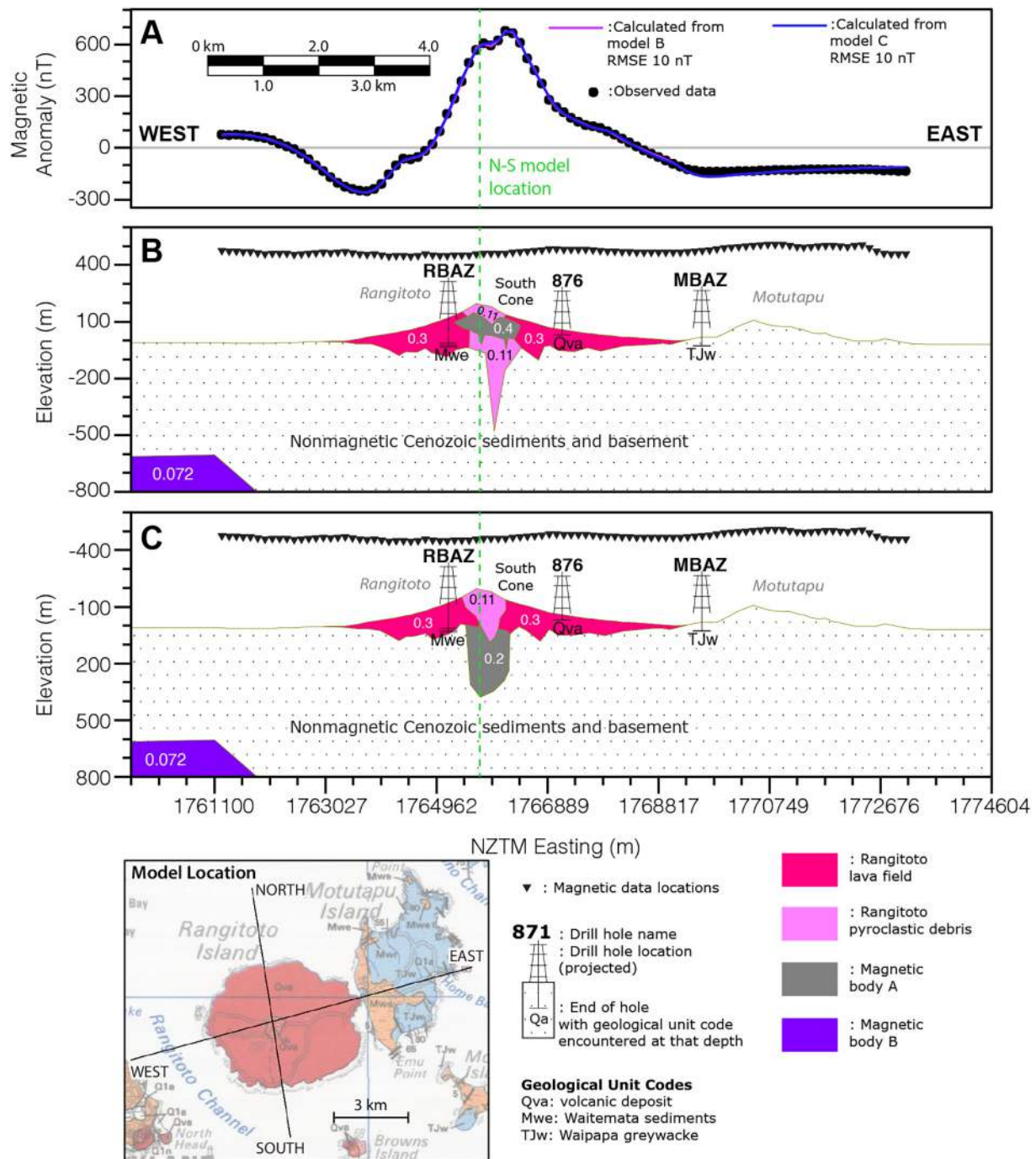
Fig. 6. (A) Observed and calculated magnetic anomaly data of west-east Rangitoto to Motutapu Islands transect. Grey line marks 0 nT. (B) and (C) are two end-members of the 2.5D models of subsurface susceptibility distribution below the transect. Legend and locator map to the models are below (C). True offline well and data point elevations have been projected onto the 2D topographic surface shown.
