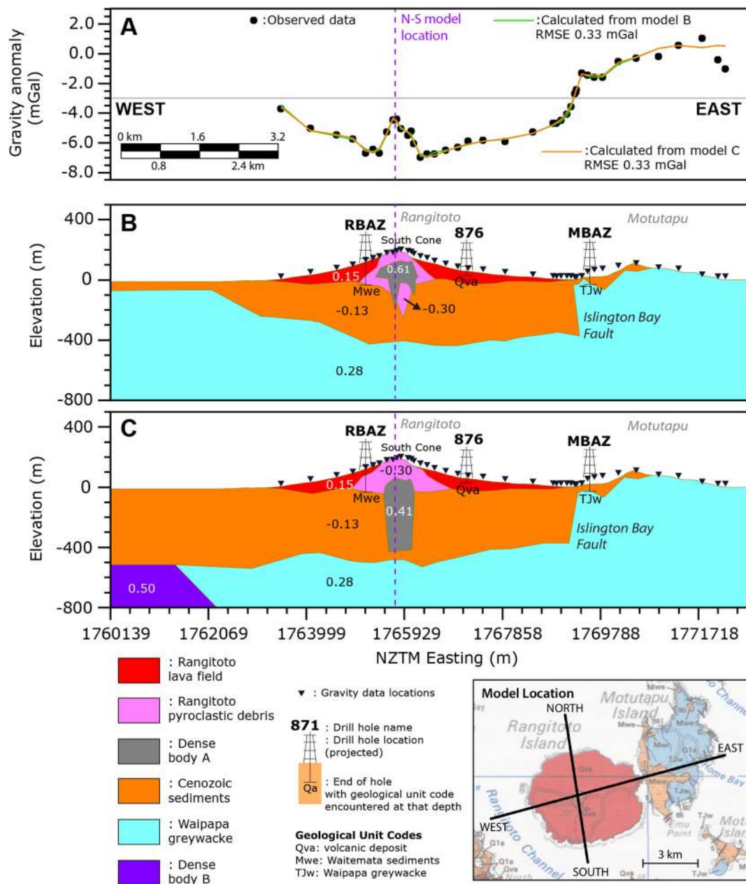
Fig. 5. (A) Observed and calculated gravity anomaly data of west-east Rangitoto to Motutapu Islands transect. The grey line marks -3 mGal. (B) and (C) are two endmembers of the 2.5D models of subsurface density distribution below the transect. Density contrasts are relative to 2.39 g/cm 3 reduction density. The legend and locator map for the models are below (C). Offline wells and data point elevations have been projected onto the 2D topographic surface shown.
