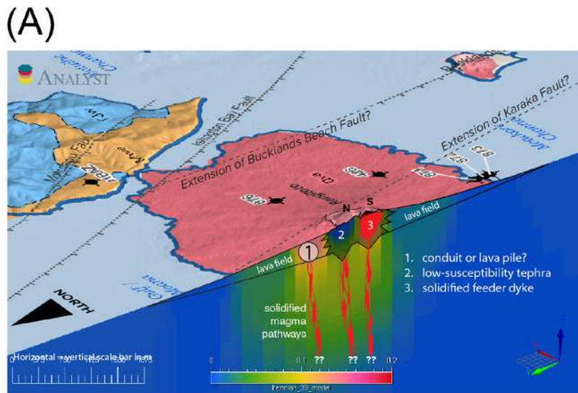
Fig. 11. A conceptual model of Rangitoto showing the geological and volcanological relevance of the models presented in this study. Figure (A) displays a schematic drawing of Rangitoto shallow subsurface volcanic features, interpreted from the north-south section of the 3D magnetic model, the compact end-member [0, 1, 1, 1]. Magnetic model cross-section is made using Geoscience ANALYST software. (B) West-east cross section of Rangitoto showing the magma captured by the a crustal structure at \sim 9 km deep, then diverted to another intersecting fracture at \sim 6 km depth and shallower, before it erupted as Rangitoto volcano. Magma diversion depth figures are indicative only. White contours show the crustal shear wave speed (in km/s) variation modelled for > 500 m depths extracted from Ensing et al. (2022). Geological map and lithology colours in this figure follow from Fig. 1.
