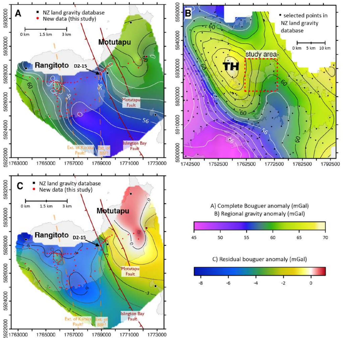
Fig. 3. (A) Complete Bouguer anomaly of the Rangitoto-Motutapu Islands, contour lines every 1 mGal. (B) Regional gravity anomaly of the Auckland Region extracted from (A), data from the New Zealand land gravity database excluding our new dataset (GNS Science, 2012; Stagpoole et al., 2021). Contour lines every 2 mGal, “TH” marks the Takapuna gravity high. (C) Residual gravity anomaly of the Rangitoto-Motutapu Islands, extracted from (A), with 1 mGal contour interval. In (A) and (C), BBF means “Bucklands Beach Fault”.
