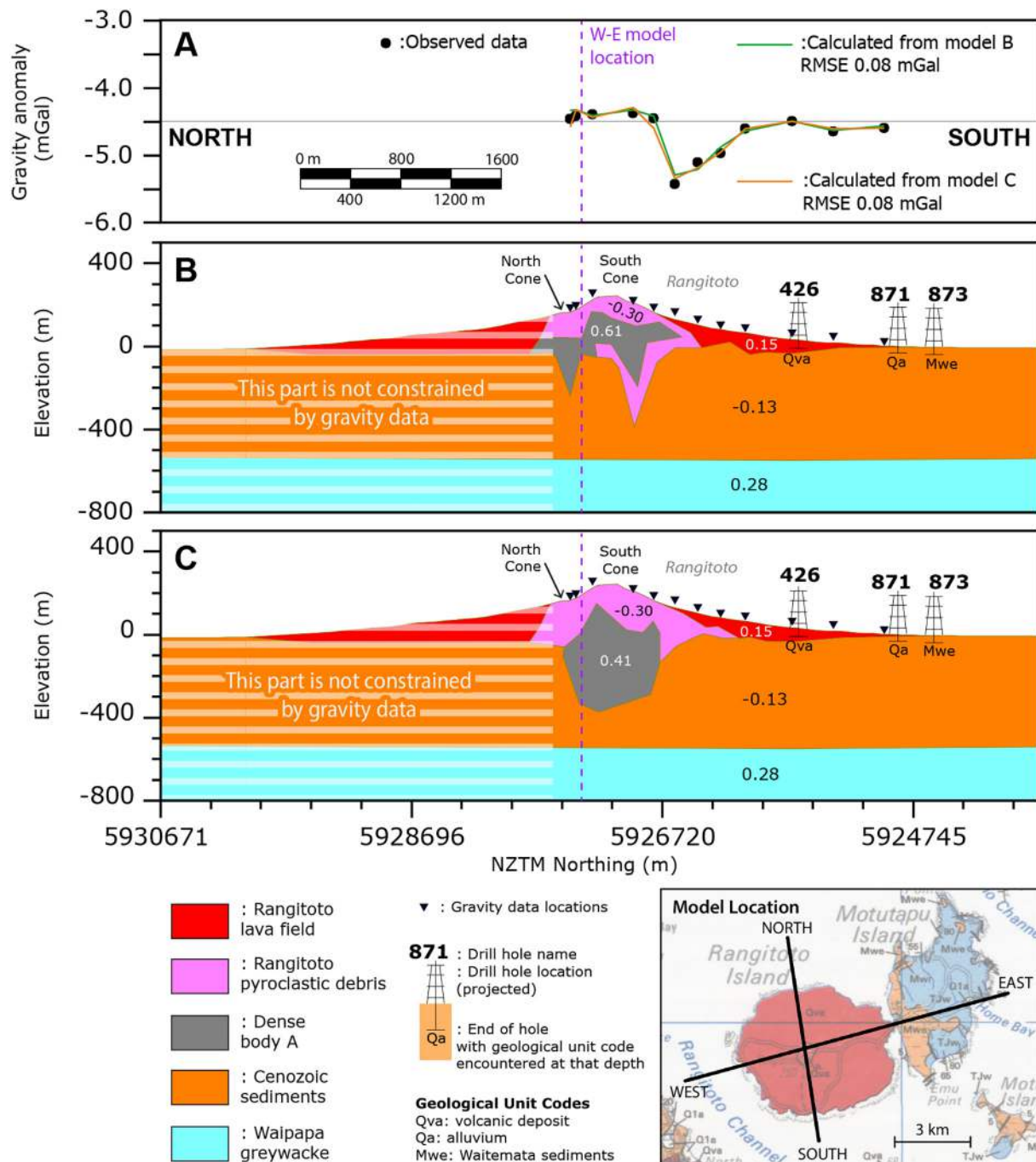
Fig. 7. (A) Observed and calculated gravity anomaly data for the north-south Rangitoto flank transect. The grey line marks -4.5 mGal. (B) and (C) are two endmembers of the 2.5D models of subsurface density distribution below the transect. Density contrasts are relative to 2.39 g/cm 3 reduction density. The legend and locator map for the models are below (C). True offline wells and data point elevations have been projected onto the 2D topographic surface shown.
