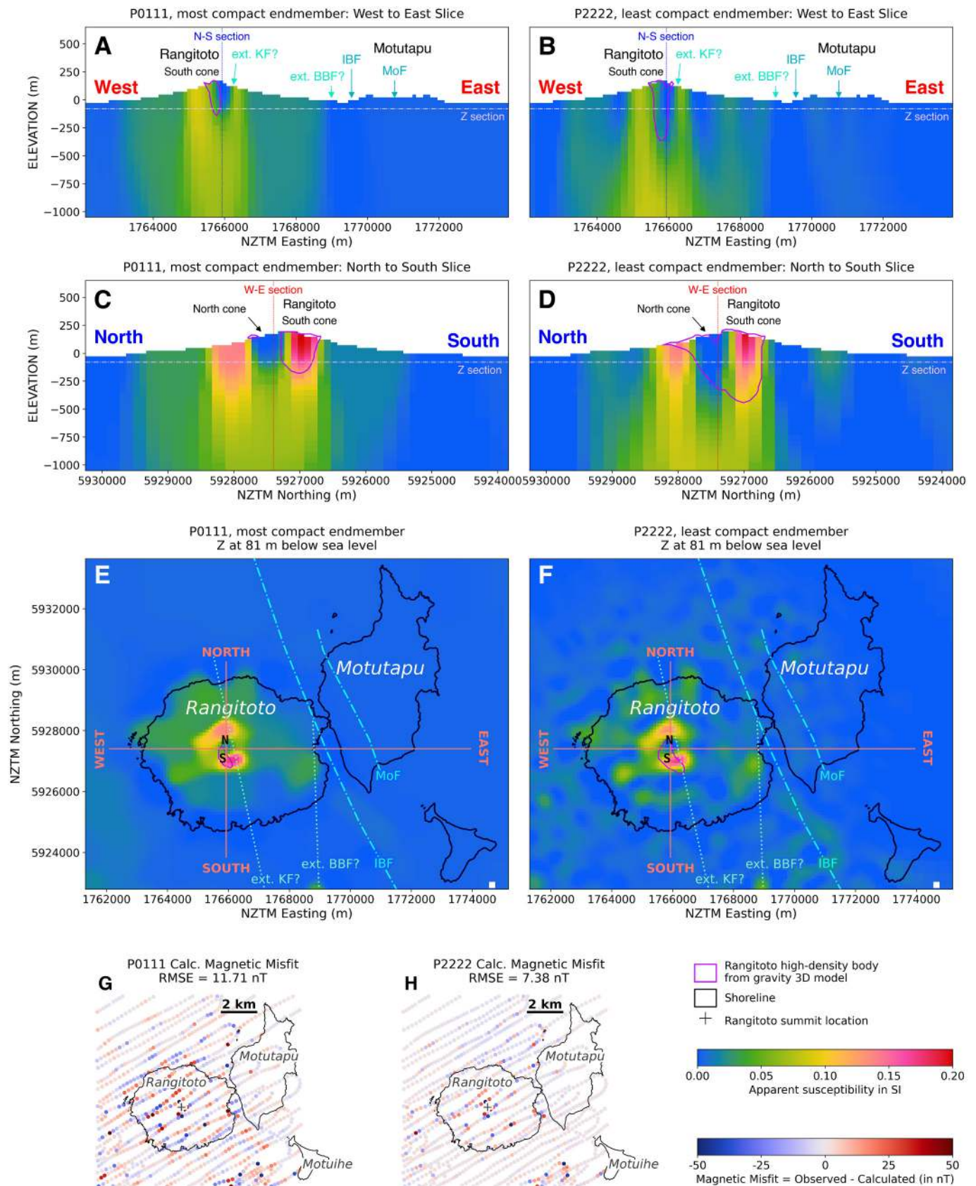
Fig. 10. Three-dimensional magnetic model of Rangitoto subsurface. Figures (A, C, E) show the west-east, north-south, and vertical slices of compact endmember [0, 1, 1, 1] of the gravity 3D models. Vertical slice is 81 m below sea level. Purple line delineates part of the 3D gravity model with > 0.035 \text{ g/cm}^3 density contrast. Compare figures (A, C, E) with figures (B, D, F) from the smooth [2, 2, 2, 2] magnetic model endmember. North and South cones of Rangitoto are marked with N and S in figures E and F. Figures (G) and (H) are the data misfit maps of the compact and smooth models, respectively. IBF: Islington Bay Fault, MoF: Motutapu Fault, ext. BBF?: extension of Bucklands Bay Fault (uncertain), ext. KF?: extension of Karaka Fault (uncertain).
